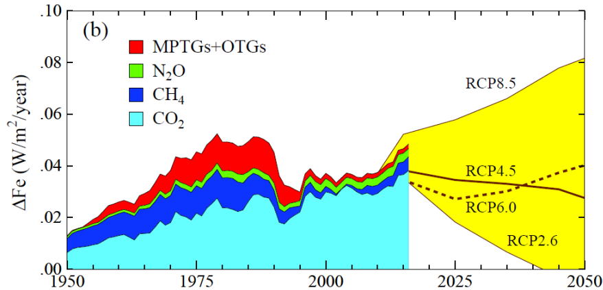
Fig. 7. Annual increase of greenhouse gas climate forcing has increased about 0.04 \text{ W/m}^2 per year for the past 50 years. RCP scenarios were defined by the Intergovernmental Panel on Climate Change (IPCC). MPTG = Montreal Protocol trace gas, OTG = Other trace gas. [Update of Fig. 8b of Burden (2017)]
