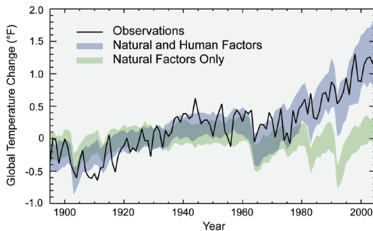
Fig. 4. Modeled and observed global temperature, from Melillo et al. (2014), who adapt the figure from Huber and Knutti (2012).
