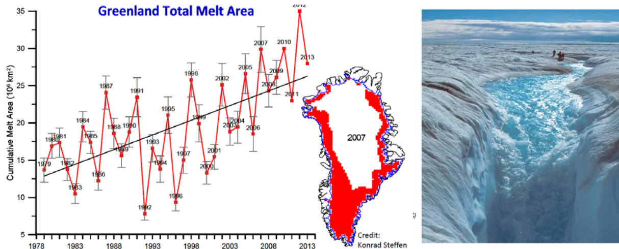
Fig. 15. Greenland area with surface melt in summer has more than doubled in recent decades. Update of chart used in Bjerknes lecture 4 , courtesy of Konrad Steffen and Russell Huff, CIRES, Univ. Colorado.
