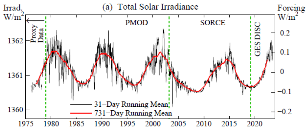
Fig. 4. Solar irradiance and climate forcing, the latter being 0.175 \times \text{irradiance change} , where 0.175 = (1 - \text{Earth's albedo})/4 , where Earth's albedo = 0.3. Data sources: Physikalisch Meteorologisches Observatorium, Davos , University of Colorado Solar Radiation and Climate Experiment , and Total Irradiance Monitor on the International Space Station (GES DISC).
