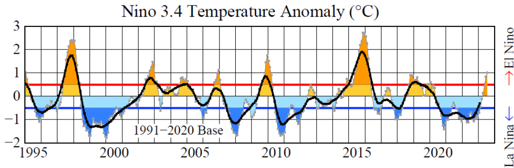
Fig. 3. Temperature in the tropical Pacific region used to define El Nino strength. El Nino (La Nina) is nominally defined to occur when Nino 3.4 is > 0.5^{\circ}\text{C} ( < -0.5^{\circ}\text{C} ).
