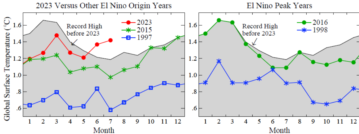
Fig. 1. Global temperature (relative to 1880-1920 mean for each month) for the 1997-98, 2015-16 and 2023-24 El Ninos. The impact of El Nino on global temperature usually peaks early in the year (El Nino Peak Year) following the year in which the El Nino originated.
